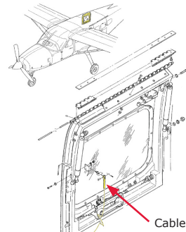
S2814-2EH Installation
