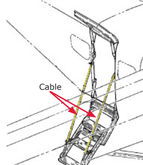
S2837-1EH or S2837-2EH Installation
