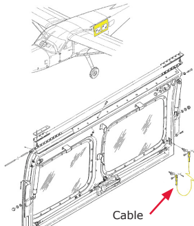
S2814-1EH Installation
