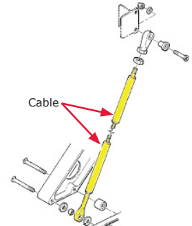
S2837-1EH or S2837-2EH Installation
