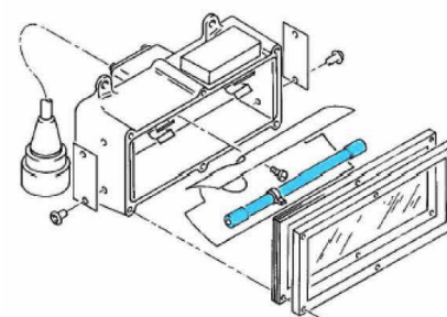
Strobe Light Assembly Lamp P/N 29210A2140055X
