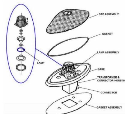
Anti-Collision Light Assembly Lamp P/N R25 2 2013A
