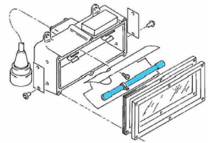
Strobe Light Assembly Lamp P/N 29210A2140055X
