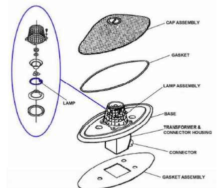
Anti-Collision Light Assembly Lamp P/N R25 2 2013A
