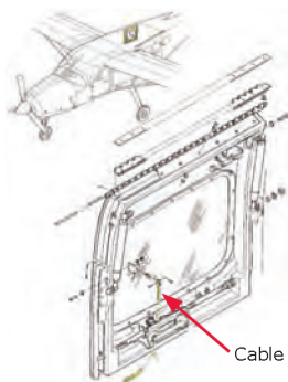
S2814-2EH Installation
