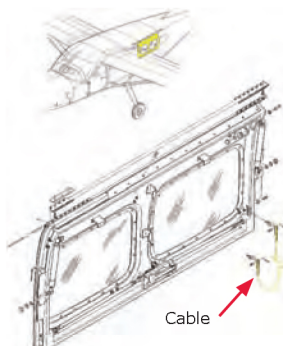
S2814-1EH Installation
